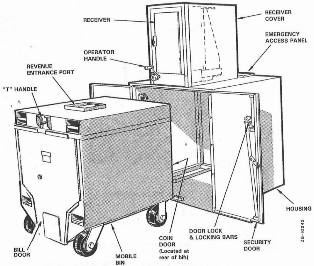
Figure A2-1. Mobile Revenue Collection System
