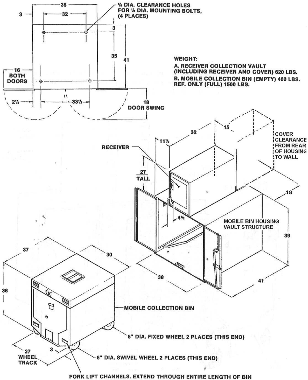
Figure A2-2. Dimensions for Receiver, Housing, & Bin
